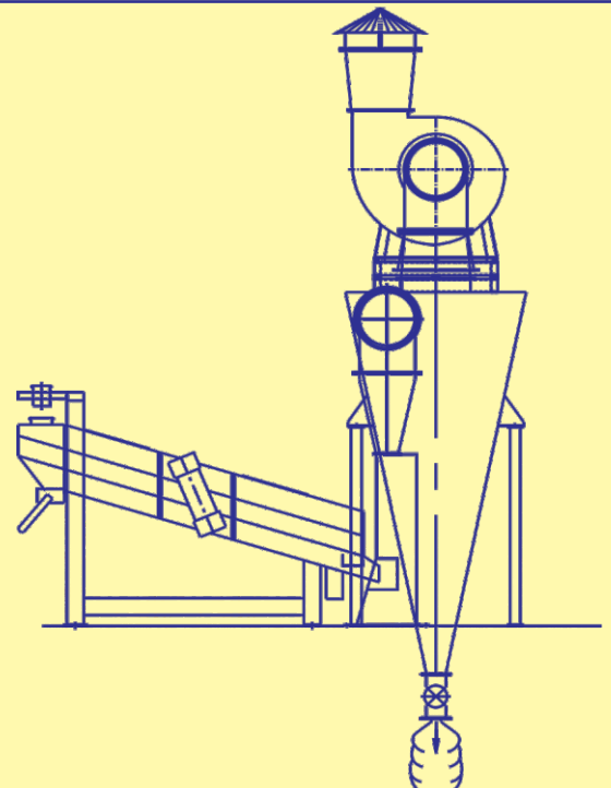
Machine with Cyclone, Blower & Rotary Valve
